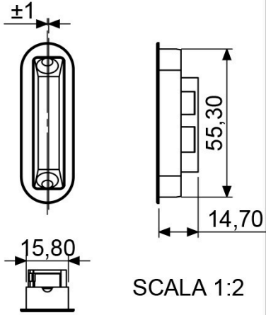
general dimension striking plate without cover
