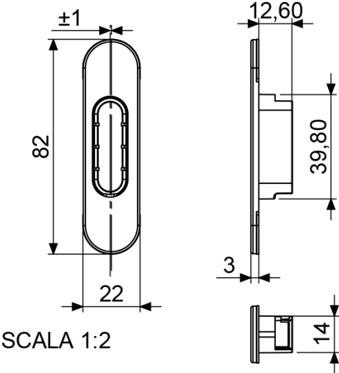
general dimension striking plate with cover
