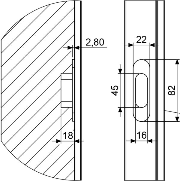
general dimension striking plate with cover
