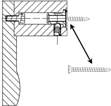
SURFACE MOUNTED
